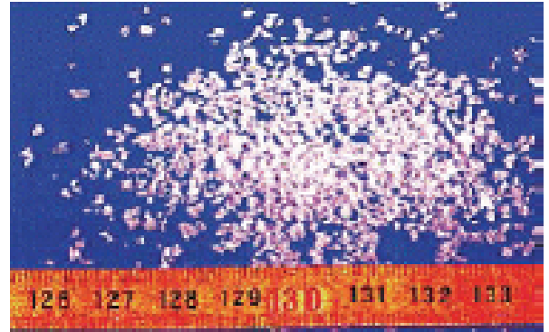
Crystalline tri-acetone tri-peroxide (TATP)
